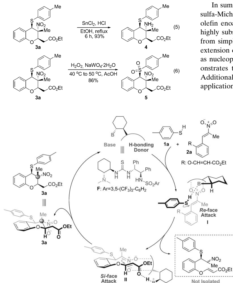
Scheme 1. Proposed reaction pathway for the cascade sequence.
