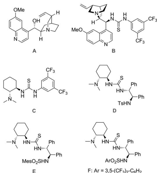
Figure 2. Bifunctional organocatalysts examined in this study. Mes = 2,4,6-trimethylphenyl, Ts = 4-toluenesulfonyl.
