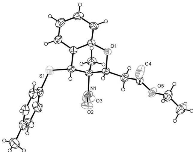
Figure 3. X-ray crystal structure of compound 3a . The thermal ellipsoids are drawn at 30% probability.
